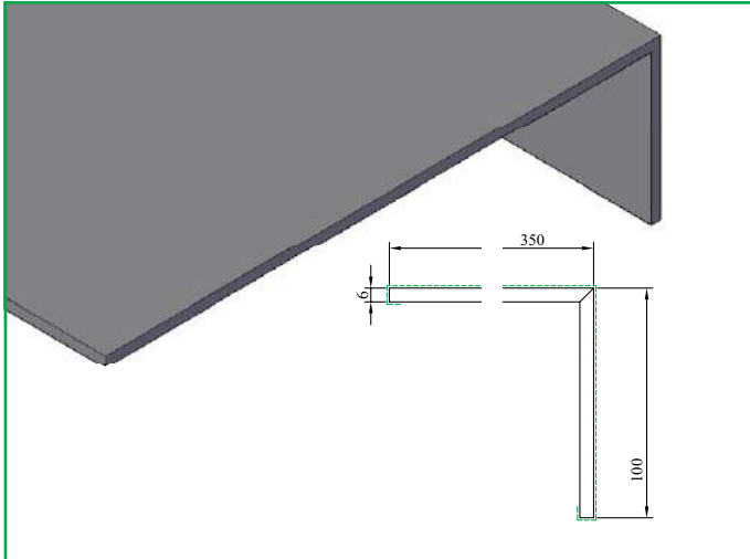
LK 600 Leidingkoker 6x100x350 mm
